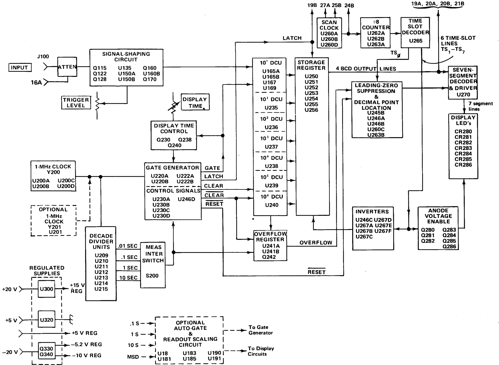
Fig. 2-1. DC 501 Block Diagram.
