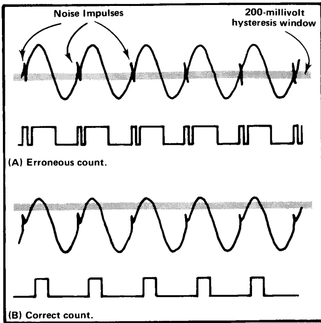
Fig. 1-2. Two examples of triggering circuit output showing how proper adjustment of TRIGGERING LEVEL control can avoid an erroneous count.
